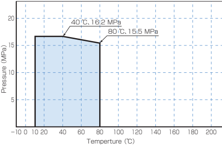
Temperature - Pressure Rating
